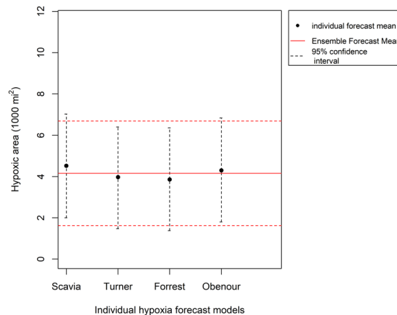
Figure 1. The 2023 NOAA ensemble forecast mean and 95% confidence interval 1 (red). The corresponding individual model means and 95% confidence intervals 1 are shown in filled circles with error bars.
