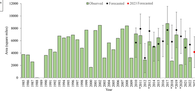
Fig 3. Observed hypoxic area (1985–2022) and forecast ensemble record interval (2010–2023). Green bars are observed hypoxic area (in square miles) measured by the LUMCON mid-summer cruise overlaid with the forecast ensemble predictions (filled circles) with 95% confidence interval 1 . The 2023 forecast is the red filled circle. The annual forecasts are made assuming normal weather conditions with asterisks indicating atypical years prior to the cruise which impacted the observed size (*high winds prior to the cruise).
