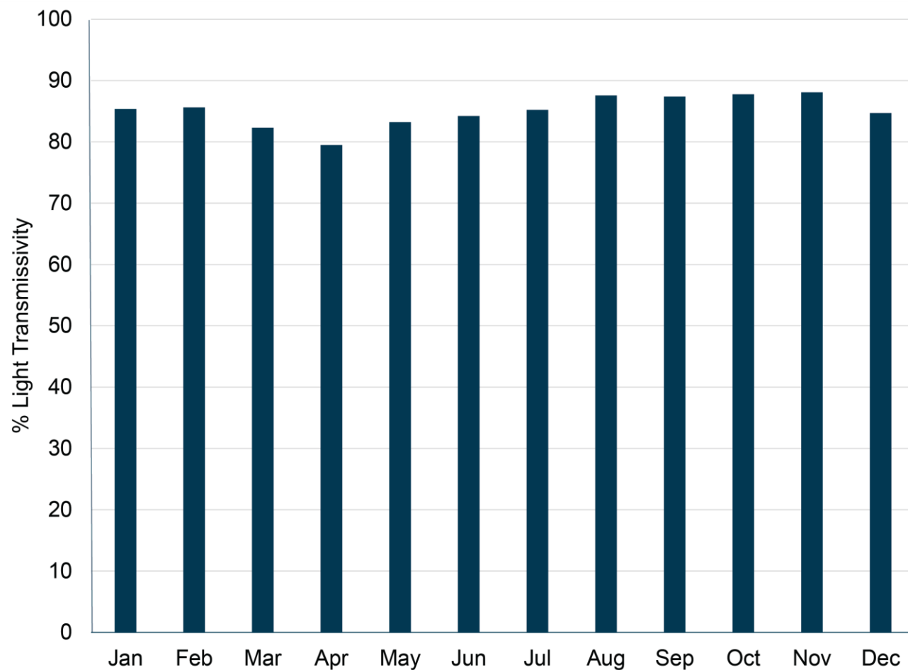
Figure 3.96. Cluster CN1 monthly climatological mean (2010 - 2018) for percent light transmissivity at 1 m produced by Visible Infrared Imaging Radiometer Suite 750-m data.
