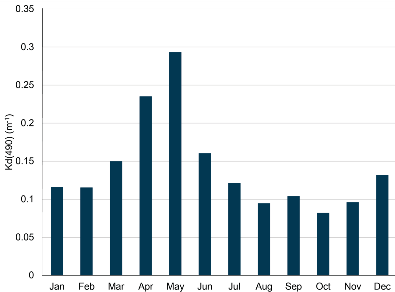
Figure 3.57. Cluster N1 monthly climatological mean (2010 - 2018) for light attenuation K_d(490) at the sea surface produced by Visible Infrared Imaging Radiometer Suite 750-m data.
