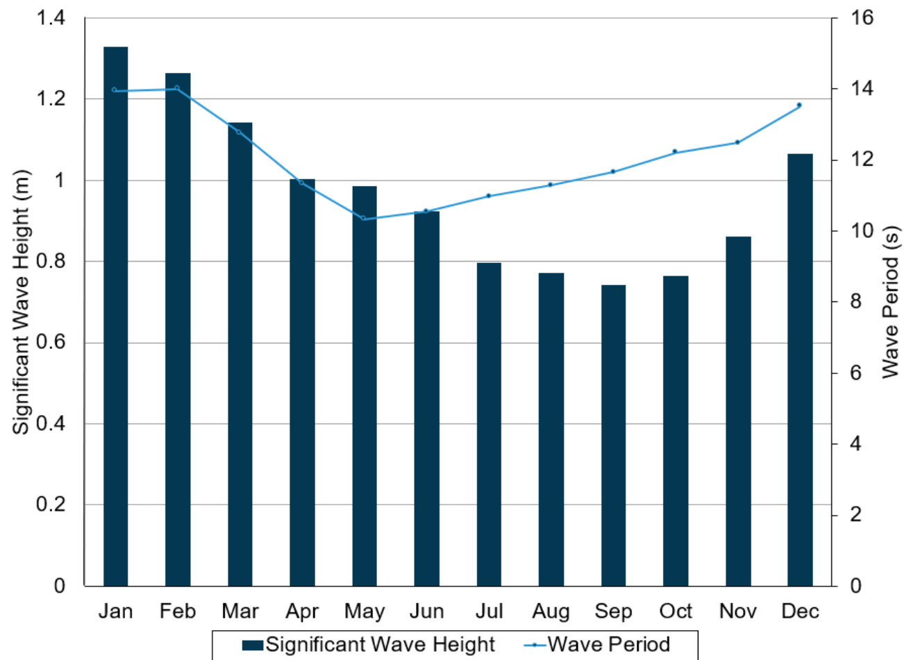
Figure 3.72. Wave height and period for cluster N2 from the Pacific Northwest National Laboratory Simulating WAVes Nearshore wave model (1979 - 2010).
