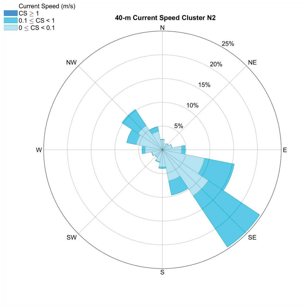
Figure 3.70. Ocean current magnitude and direction for cluster N2 at 40-m depth. The rose diagram provides percent occurrence for each current speed (CS) category. Current flow is in the direction of the compass heading. Data are from the California Regional Ocean Modeling System (2016 - 2020).
