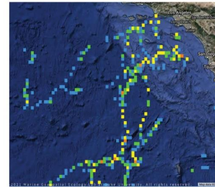
Figure 30. Summary of loggerhead locations reported in the OBIS Seamap database ( https://seamap.env.duke.edu/species/173830 ).
