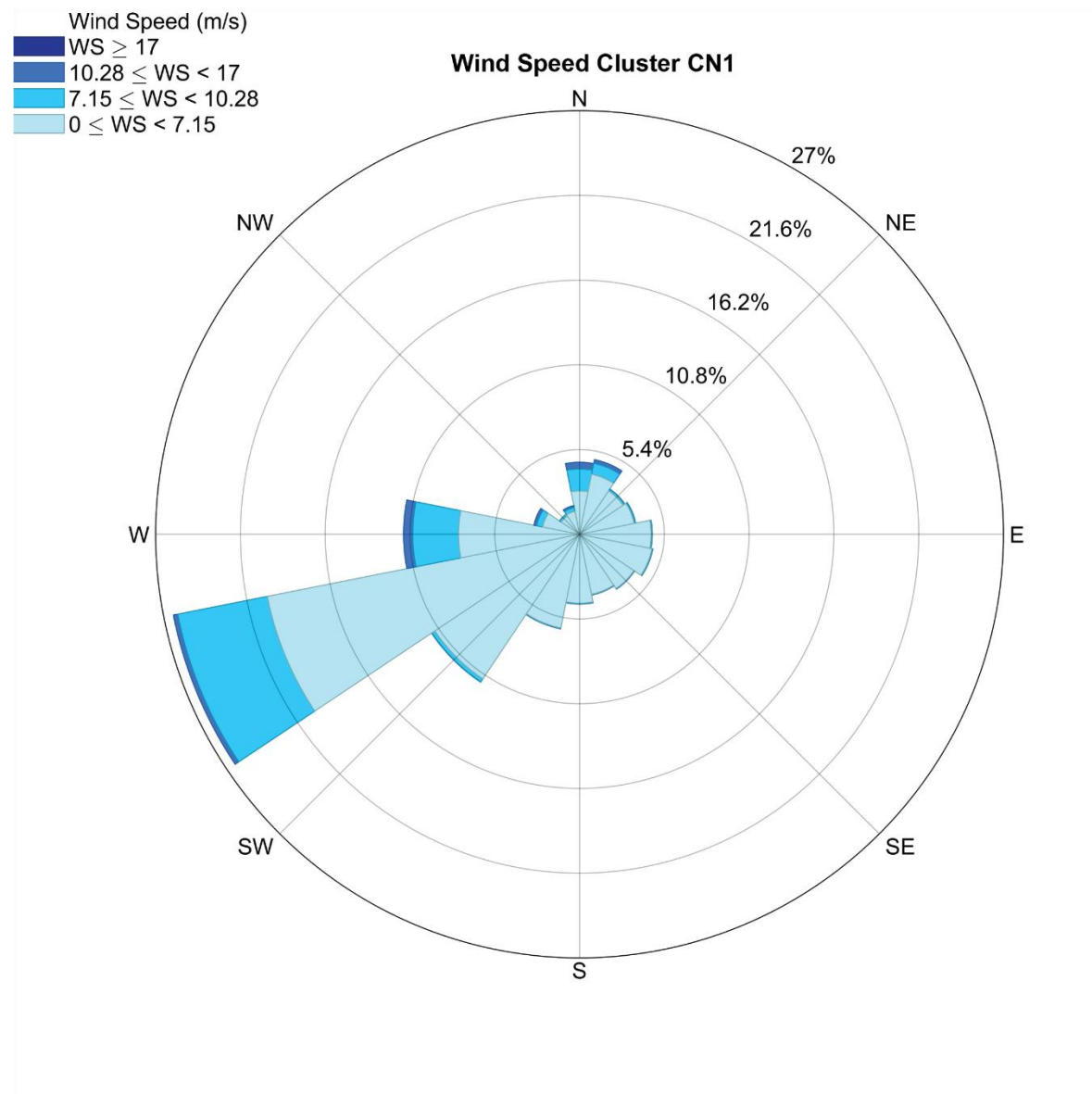
Figure 3.91. Wind velocity and direction at 10-m above sea level for cluster CN1. The rose diagram provides percent occurrence for each wind speed (WS) category. Wind direction is displayed as the origin. Wind data are from the Coupled Ocean/Atmosphere Mesoscale Prediction System model (2016 - 2020).
