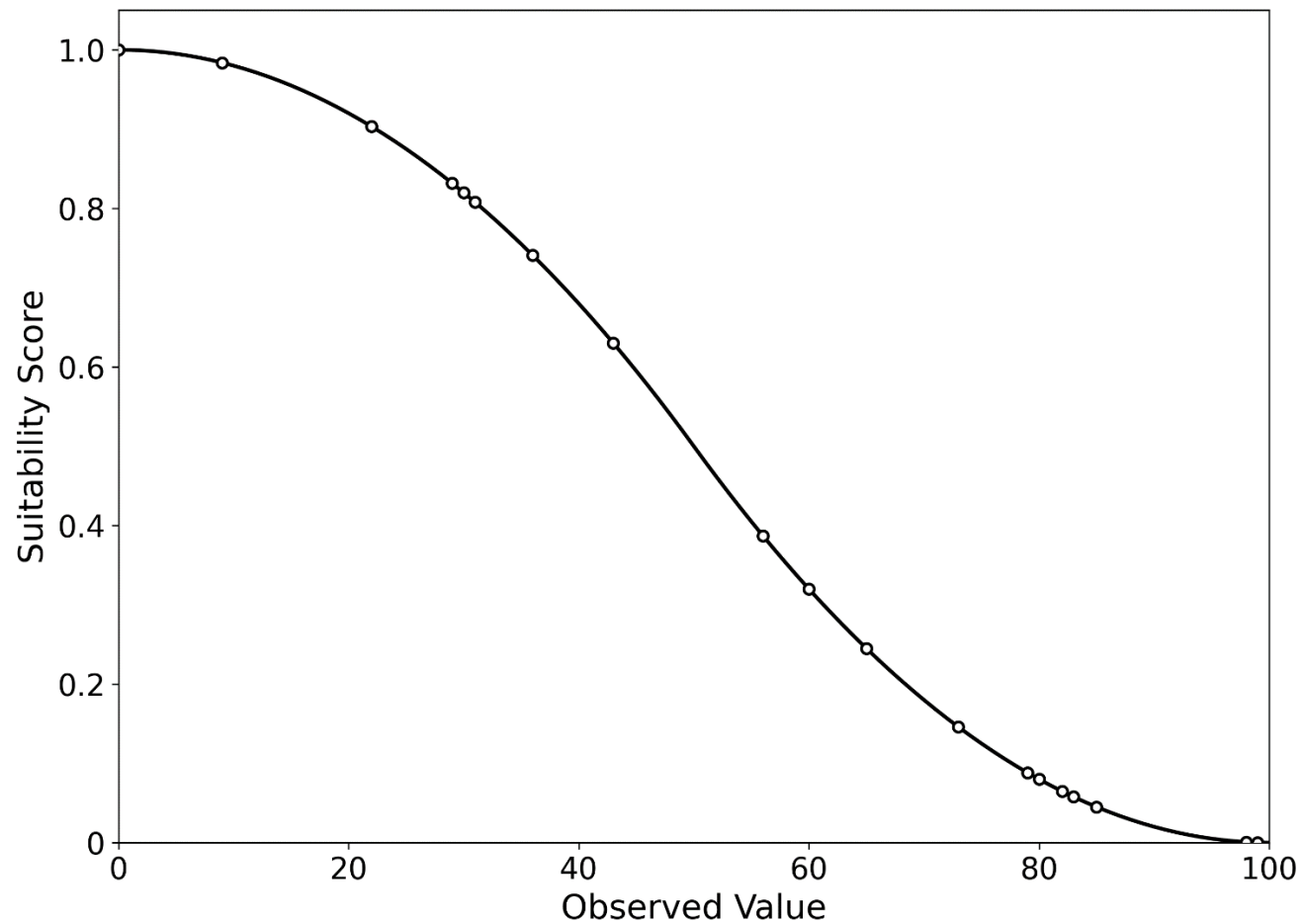
Figure 2.7. Example of a hypothetical Z-shaped membership function, with the minimum observed value being 0 and the maximum observed value being 99. However, the total range of the function goes to 100, as 1 was added to 99 when creating the function to ensure no observed values would be rescaled to 0. For example, the points on the line indicate the intersection of an observed value (e.g., vessel traffic) and the corresponding score to which it would be rescaled from the function.
