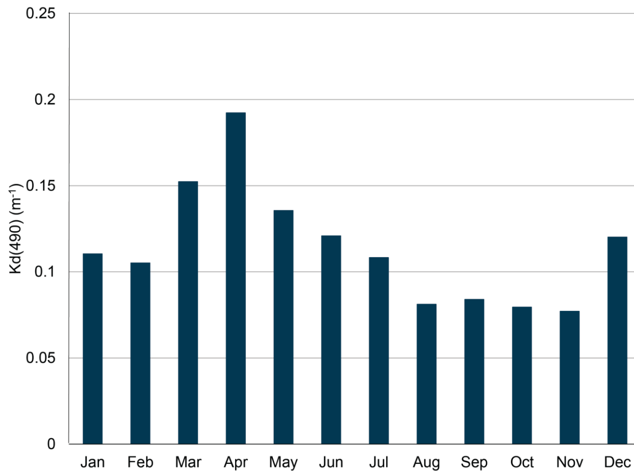
Figure 3.95. Cluster CN1 monthly climatological mean (2010 - 2018) for light attenuation, K_d(490) at the sea surface produced by Visible Infrared Imaging Radiometer Suite 750-m data.
