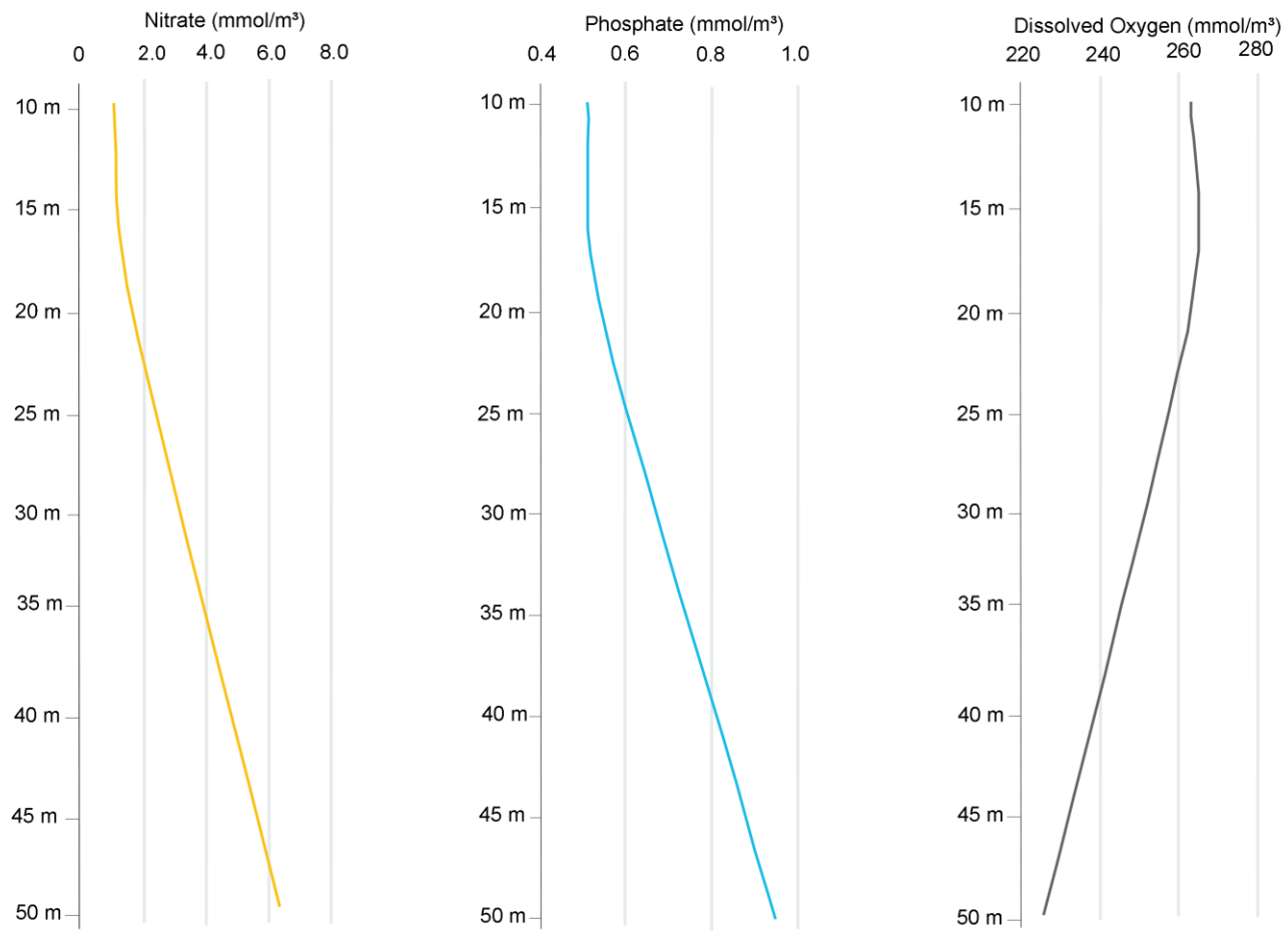
Figure 3.55. Cluster N1 concentration of nitrate, phosphate, and dissolved oxygen at depth (Kessouri et al. 2021).
