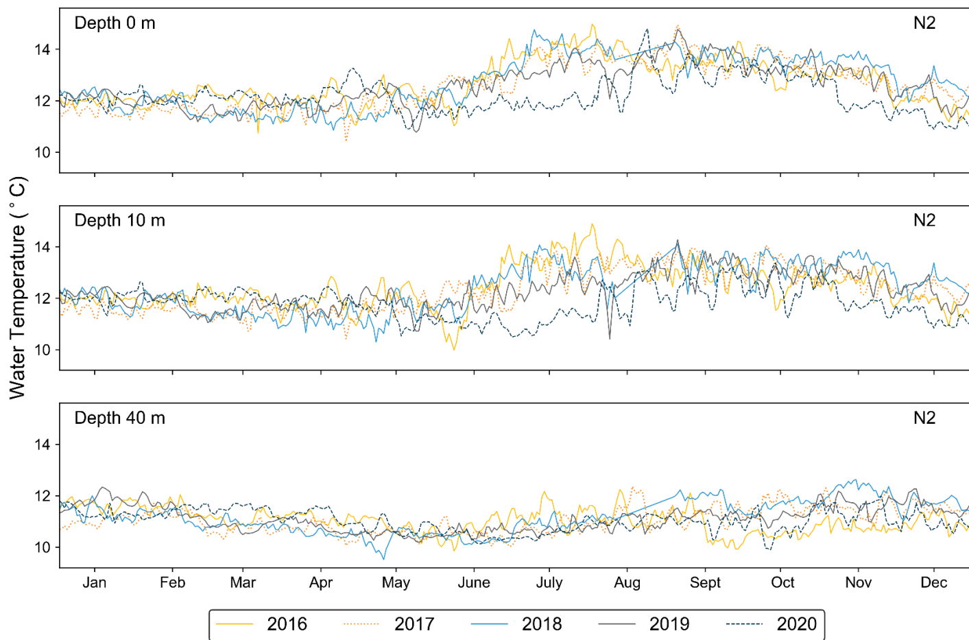
Figure 3.67. Water temperature at 0 m, 10m, and 40 m for cluster N2 from the California Regional Ocean Modeling System model (2016 - 2020).
