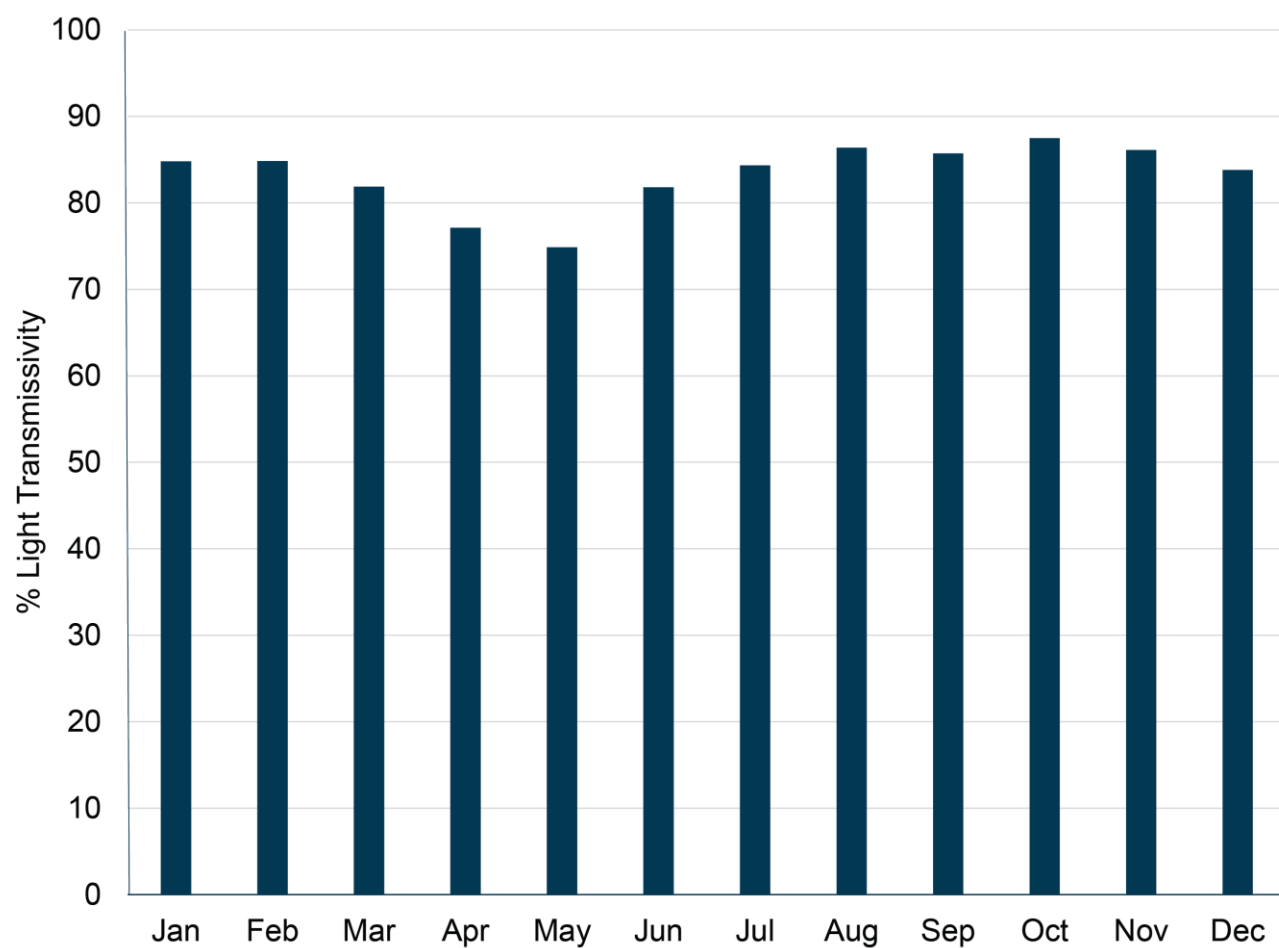
Figure 3.58. Cluster N1 monthly climatological mean (2010 - 2018) for percent light transmissivity at 1 m produced by Visible Infrared Imaging Radiometer Suite 750-m data.
