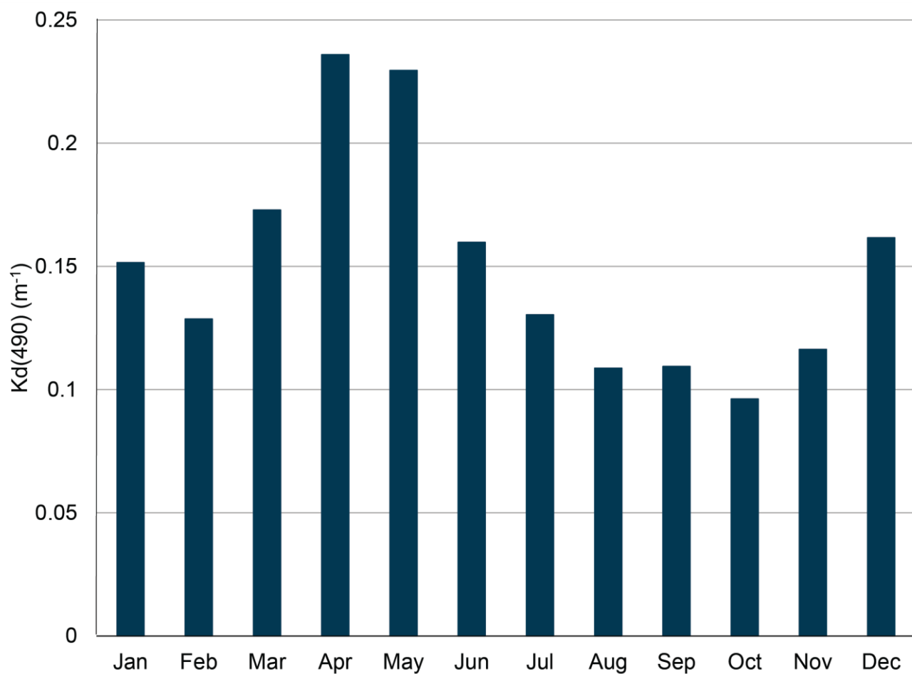
Figure 3.75. Cluster N2 monthly climatological mean (2010 - 2017) for light attenuation, K_d(490) , at the sea surface produced by Visible Infrared Imaging Radiometer Suite 750-m data.
