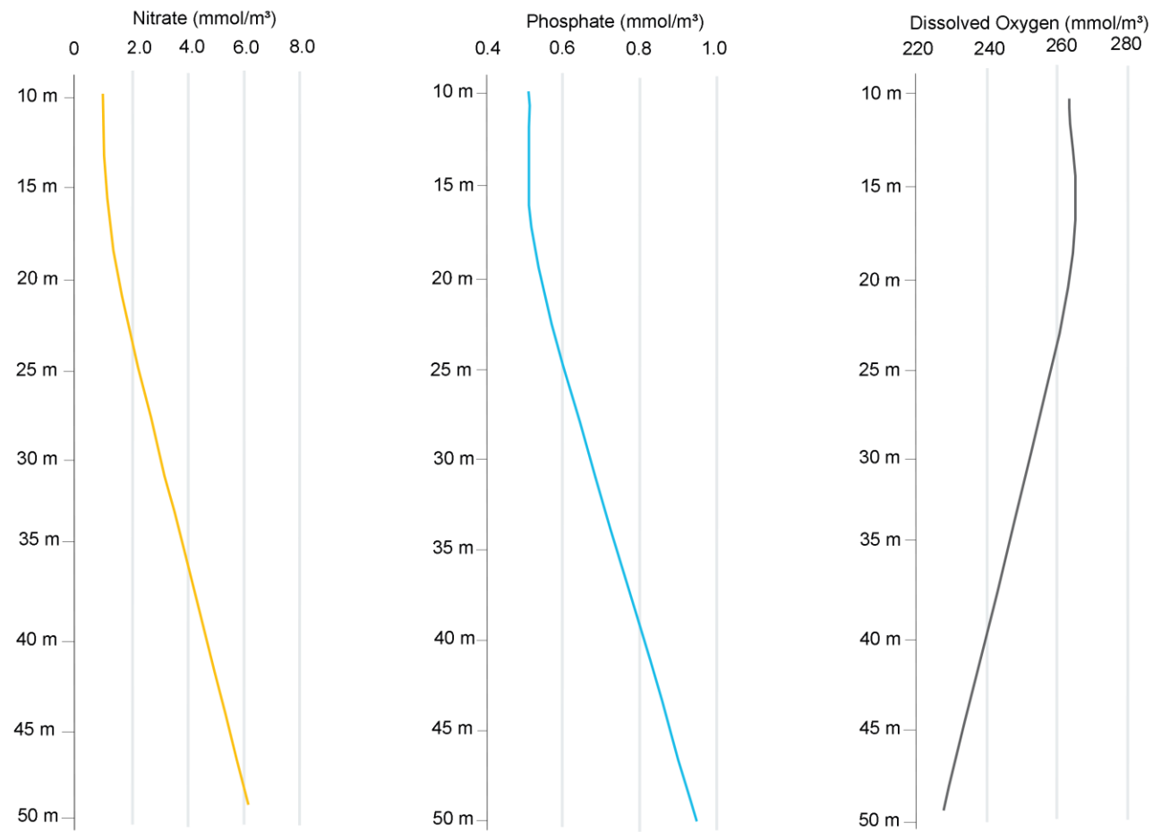
Figure 3.73. Cluster N2 concentration of nitrate, phosphate, and dissolved oxygen at depth (Kessouri et al. 2021).
