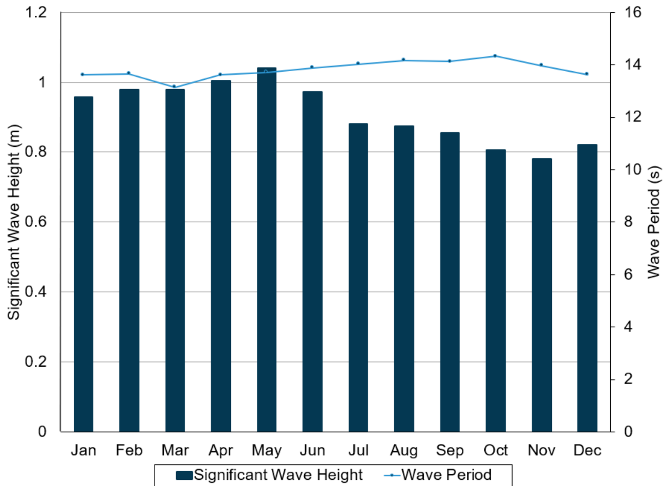
Figure 3.92. Wave height and period for cluster CN1 from the Pacific Northwest National Laboratory Simulating WAVes Nearshore wave model (1979 - 2010).
