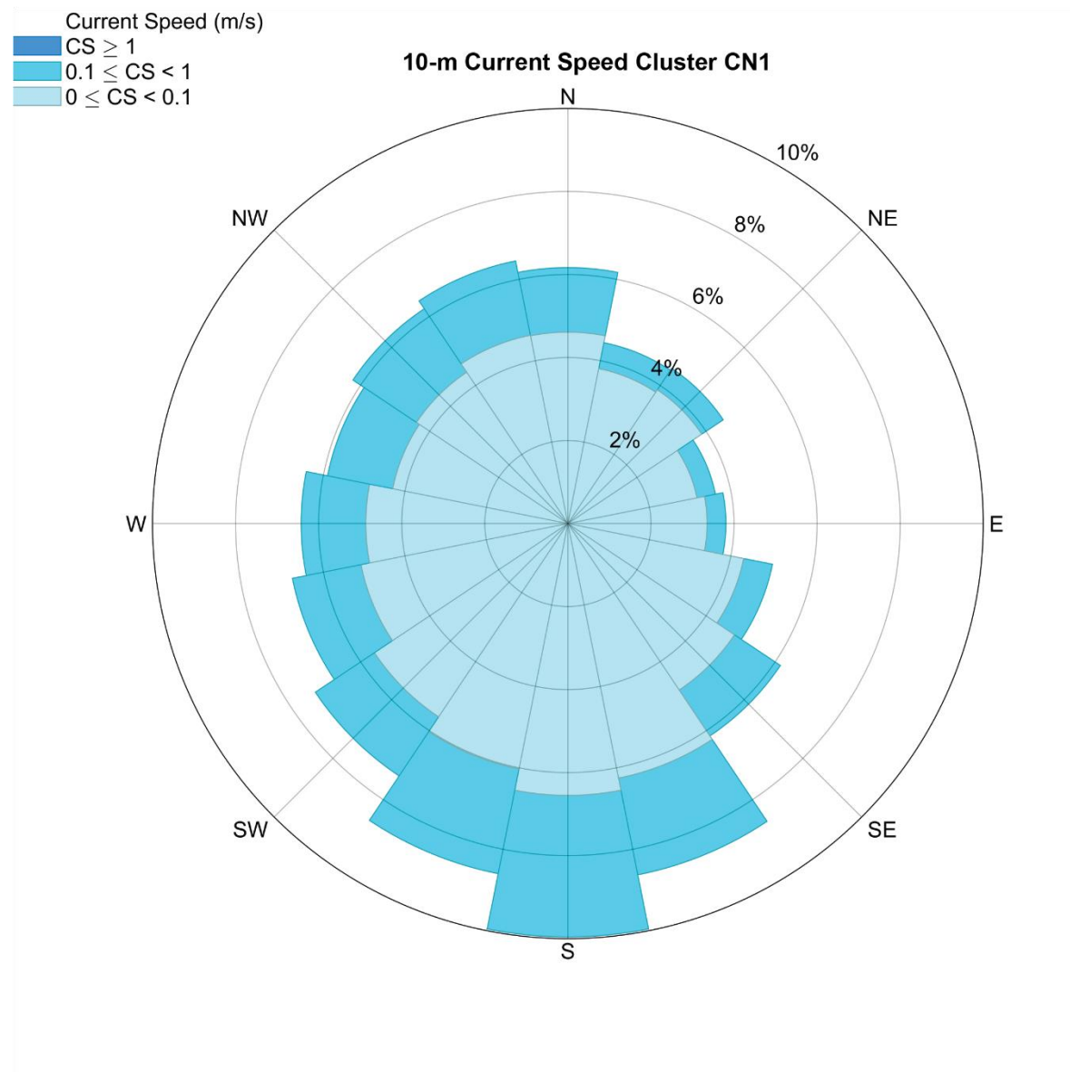
Figure 3.89. Ocean current magnitude and direction for cluster CN1 at 10-m depth. The rose diagram provides percent occurrence for each current speed (CS) category. Current flow is in the direction of the compass heading. Data are from the California Regional Ocean Modeling System (2016 - 2020).
