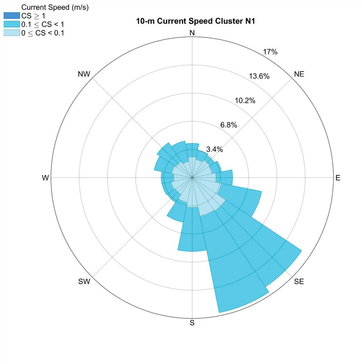
Figure 3.51. Ocean current magnitude and direction for cluster N1 at 10-m depth. The rose diagram provides percent occurrence for each current speed (CS) category. Current flow is in the direction of the compass heading. Data are from the California Regional Ocean Modeling System (2016 - 2020).
