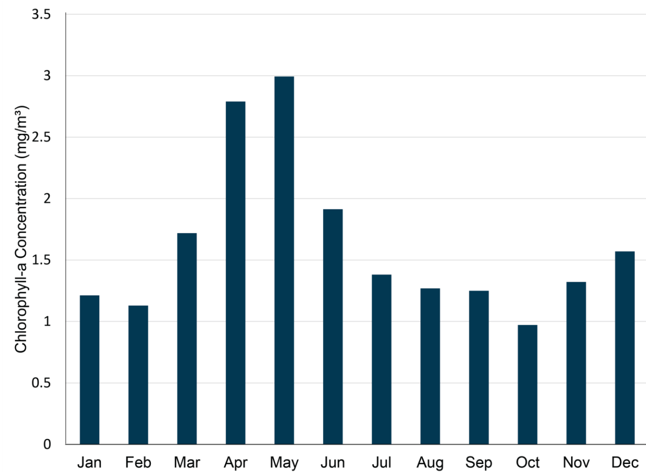
Figure 3.74. Cluster N2 monthly climatological mean (2016 - 2020) concentration of chlorophyll-a (mg/m³) at the surface from Visible Infrared Imaging Radiometer Suite Level 3 750-m data.
