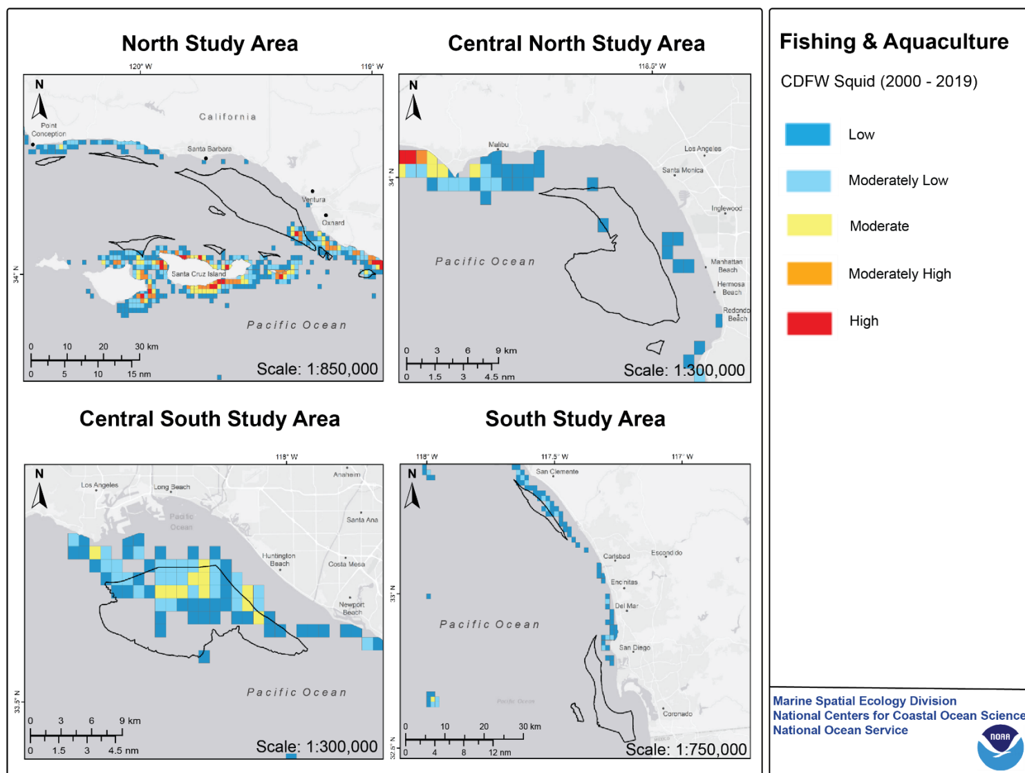
Figure 3.18. Aggregated California Department of Fish and Wildlife squid data (2000 - 2019) for the North, Central North, Central South, and South study areas. Blue colors represent lower catch estimates in the time period examined, while orange and red colors represent relatively higher catch estimates.
