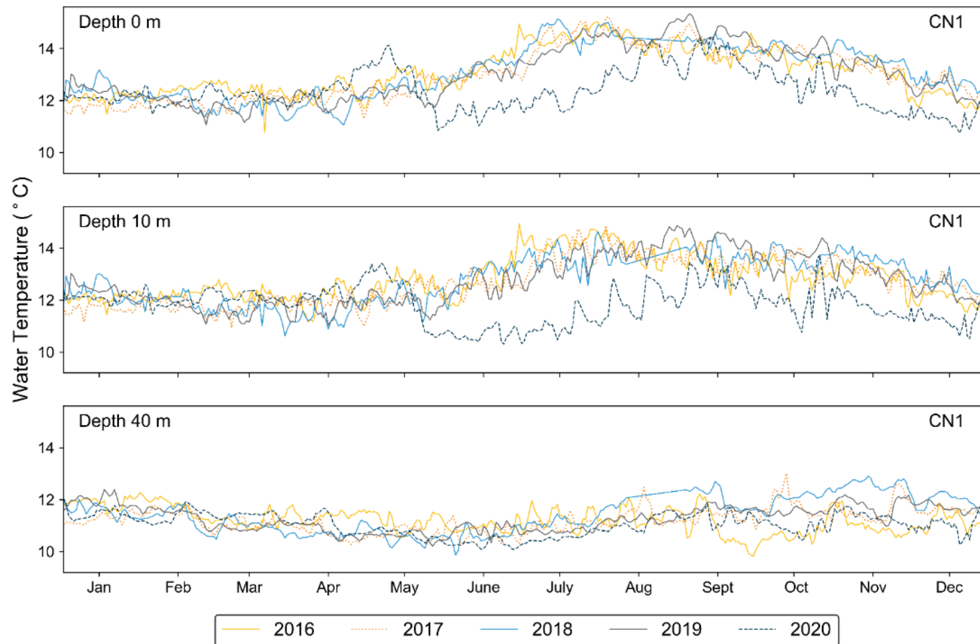
Figure 3.87. Water temperature at 0-m, 10-m, and 40-m depth for cluster CN1 from the California Regional Ocean Modeling system model (2016 - 2020).
